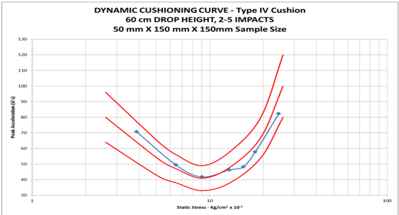
Figure 1. Dynamic Cushioning Curve of the Foam Product in comparison to Type IV Low, Nominal, and High Guidelines
