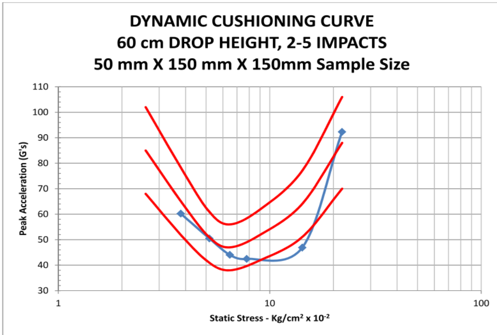
Figure 1: Dynamic Cushioning Curve of the Foam Product in comparison to Type III Low, Nominal, and High guidelines.
